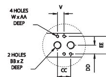
SOLENOID MOUNTING
