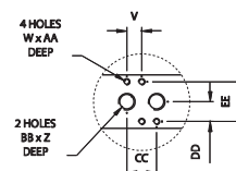
SOLENOID MOUNTING
